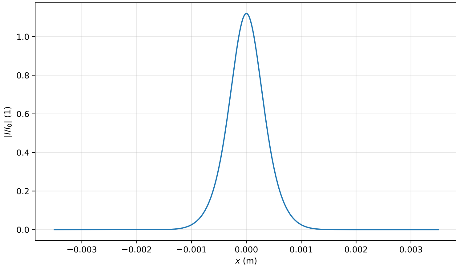
Intensity profile I(x, y = 0, z = 0.955m)/I_0 , P_{in}=0.6P_{cr} , artificial time
